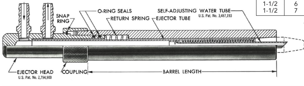
Cross-section view of holders with barrels 7/8 inch or less diameter.
