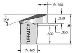
OFFSET SE-3248 Part No. 170-3248
