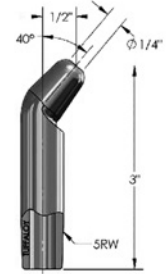
FP-2530-8 Part No. 167-5070
